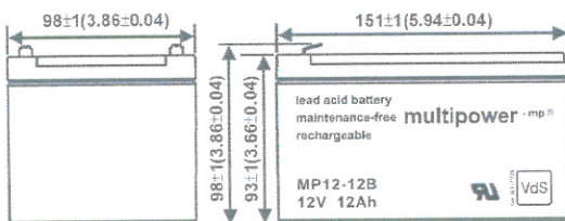
(V) FOR 12V BATTERY
